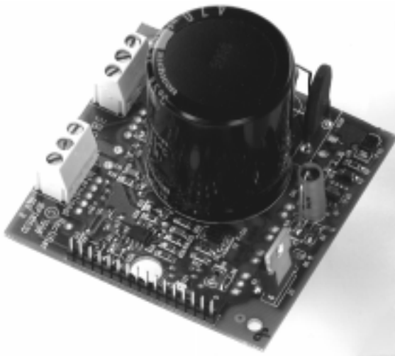
Figure 3. IRPT1060D Driver-Plus Board
